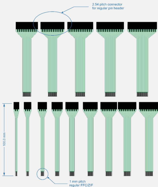
2.54 array, 2-15 ways connector house
