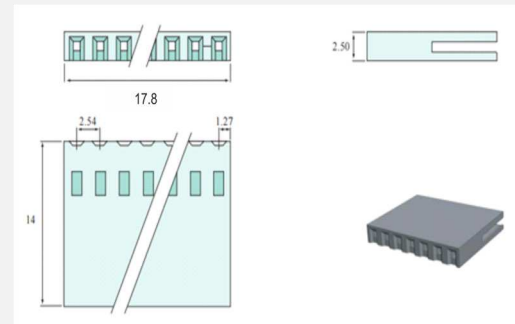
2.54 array, 2-15 ways connector house
